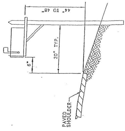
PAVED SHOULDER
